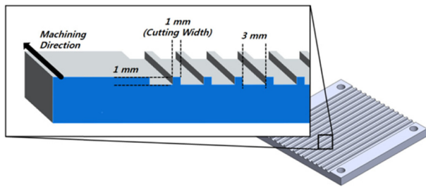
Fig. 1 Ti-6Al-4V specimen for orthogonal cutting process
