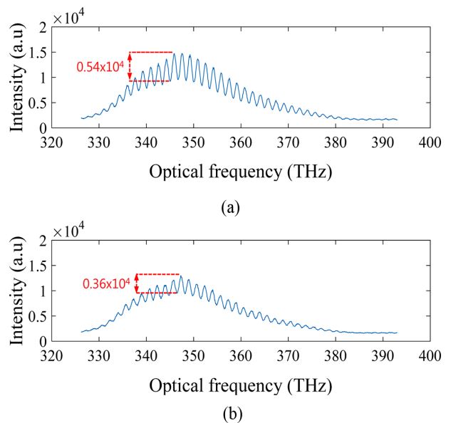
Fig. 2 Measured at same distance (90 μm) when the thickness of BK7: (a) 0 mm, (b) 0.9 mm
