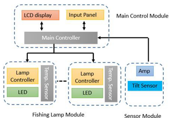
Fig. 1 Composition of an LED fishing lamp system
