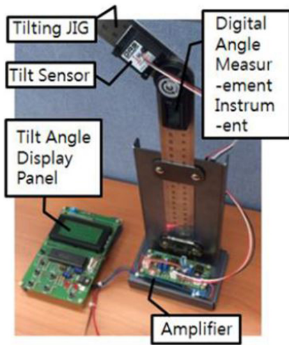
Fig. 7 Angle test bench
