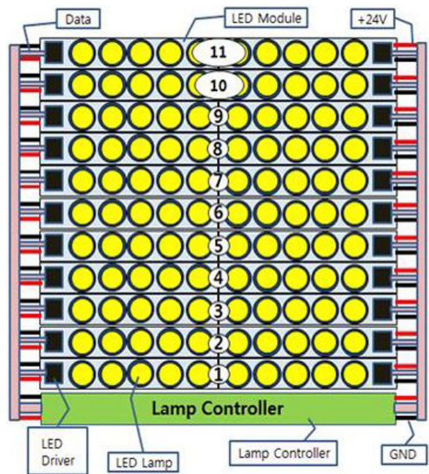
Fig. 4 Composition of a fishing lamp module
