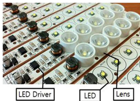
Fig. 6 Fabricated LED module
