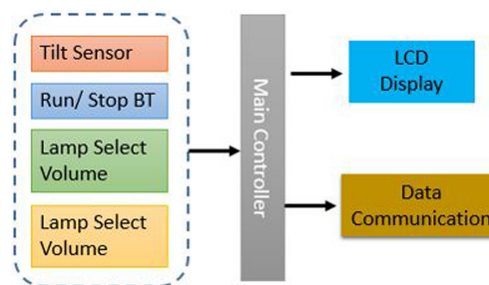
Fig. 2 Configuration and signal flow of the main control module
