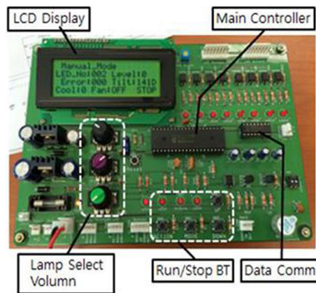
Fig. 3 Fabricated main controller module
