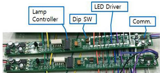
Fig. 5 Fabricated lamp controller
