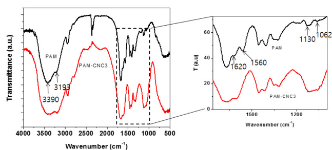
Fig. 6 FTIR spectra of pure PAM, CNC and PAM-CNC1 composite hydrogel
