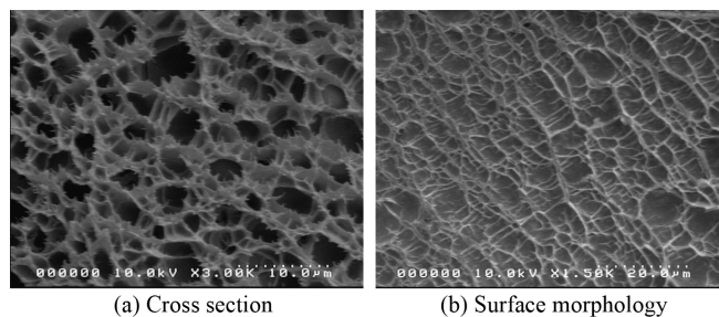
Fig. 4 SEM analysis of polyacrylamide/CNC
