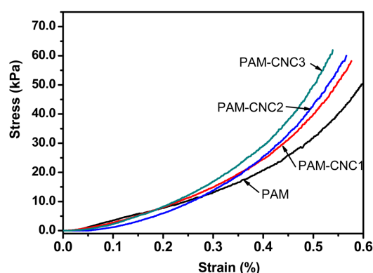
Fig. 8 Compressive stress-strain curves of different hydrogels
