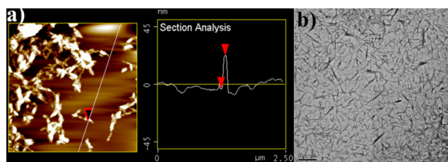
Fig. 3 Images of the isolated CNC: (a) AFM, (b) TEM
