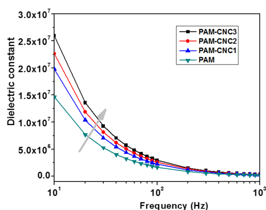
Fig. 9 Dielectric property of polyacrylamide and its composite hydrogels
