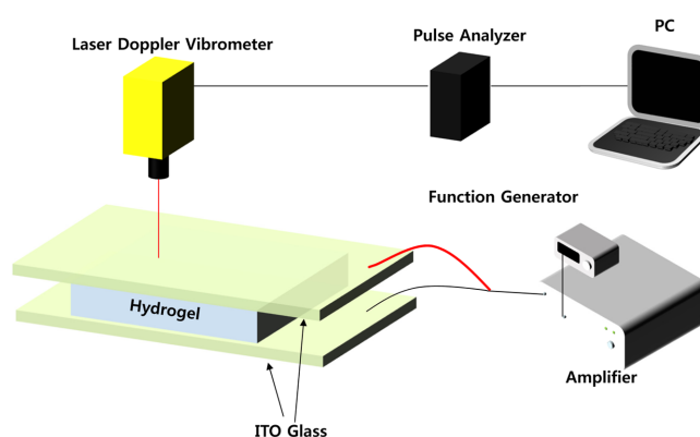
Fig. 2 Experimental setup for electro-active actuation test
