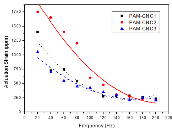
Fig. 10 Electro-Active behavior of PAM-CNC composite hydrogels
