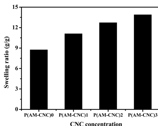
Fig. 7 Swelling ratio of PAM-CNC composite hydrogels with different CNC concentration
