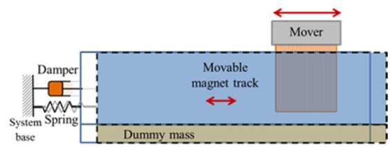
(a) Schematics of the passive RFC mechanism
