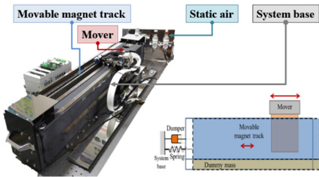
Fig. 3 An air-bearing linear motor motion stage with the passive RFC
