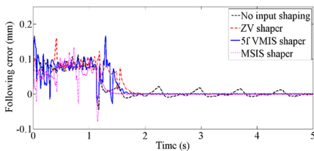
Fig. 10 Mover in-position errors of two special shaped motion profiles
