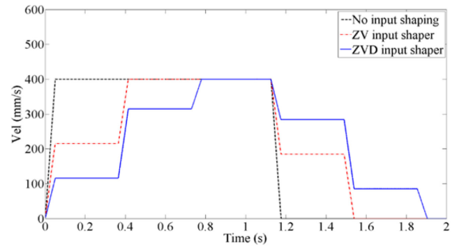
(a) Velocities of original and shaped input motion profiles
