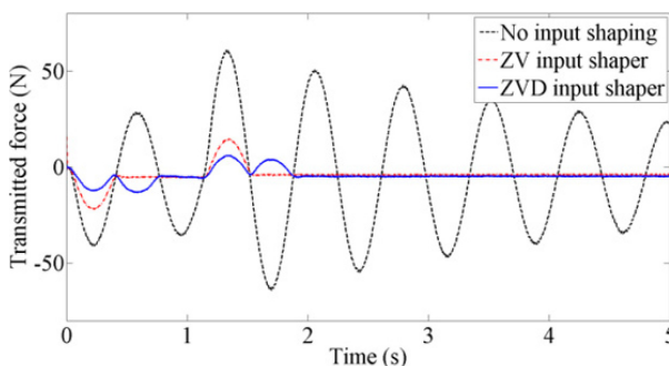
Fig. 7 Transmitted force: original and shaped input motion profiles
