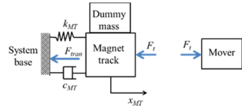
(b) Schematic model of the passive RFC mechanism
