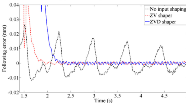
(c) Mover in-position errors: detailed view
