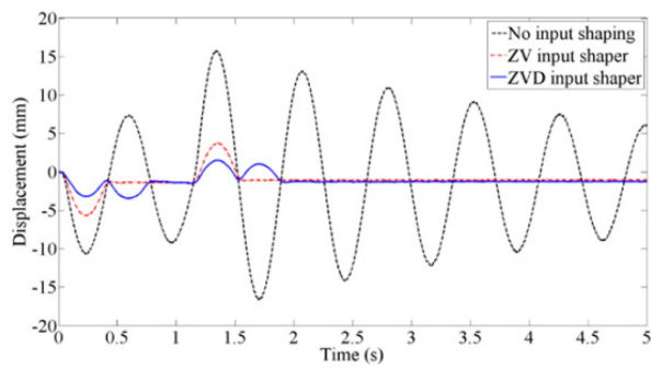
(a) Magnet track oscillations
