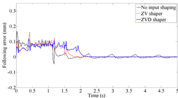
(b) Mover in-position errors
