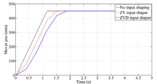
(b) Positions of original and shaped input motion profiles
