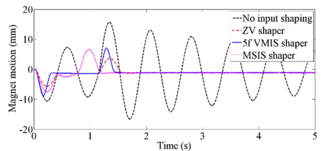
Fig. 9 Magnet track oscillations of two special shaped motion profiles
