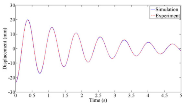
Fig. 4 System identification of modal parameters of the passive RFC mechanism
