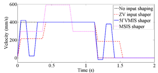
Fig. 8 Two special shaped motion profiles to compensate delayed rise time
