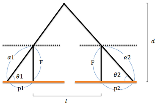
Fig. 8 Stereo triangulation
