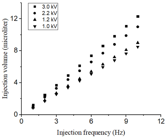
Fig. 9 Drug solution injection volume per second with respect to the injection frequency
