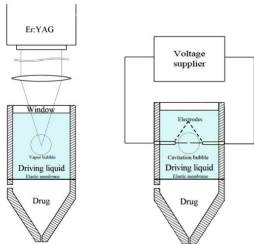
Fig. 1 Schematic of a underwater spark discharging power sources and drug chamber nozzles attached to a pressure chamber
