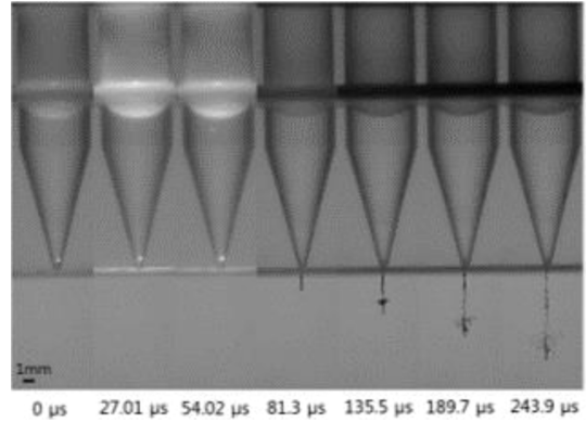
Fig. 7 The sequential images of ejecting microjets: spark-induced microjet
