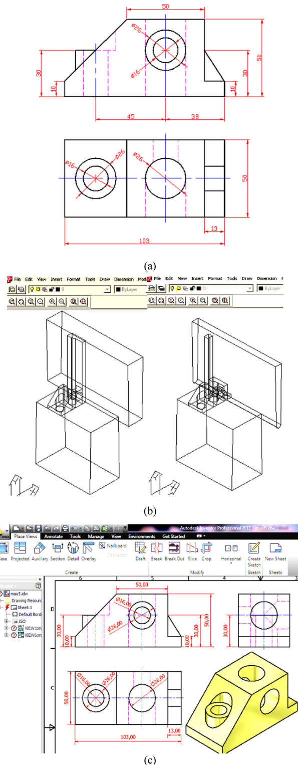
Fig. 4 (a) Drawing of 2 views, (b) 3D Solid creation, and (c) Test of resulting Solid accuracy
