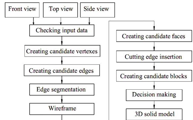
Fig. 1 Block diagram of a typical B-Rep based 3D model reconstruction method
