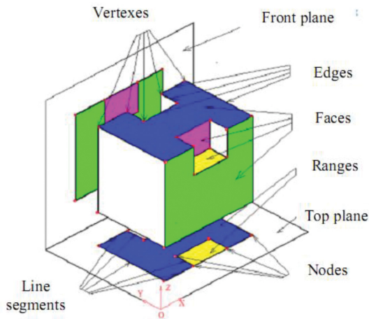
Fig. 2 Definitions in 2D View and 3D object
