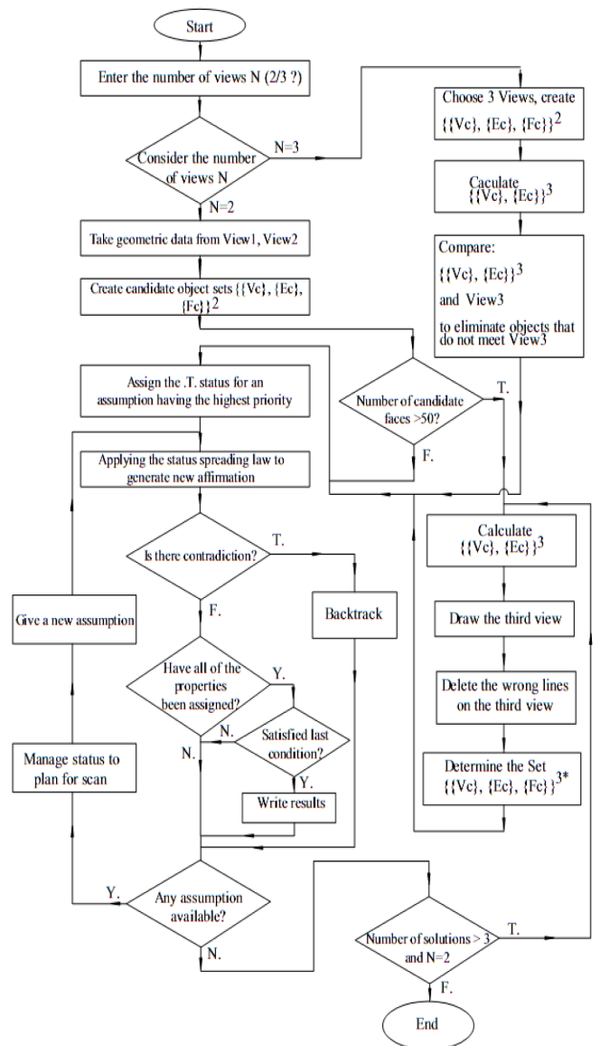
Fig. 3 Algorithm block diagram of flexible reconstruction system
